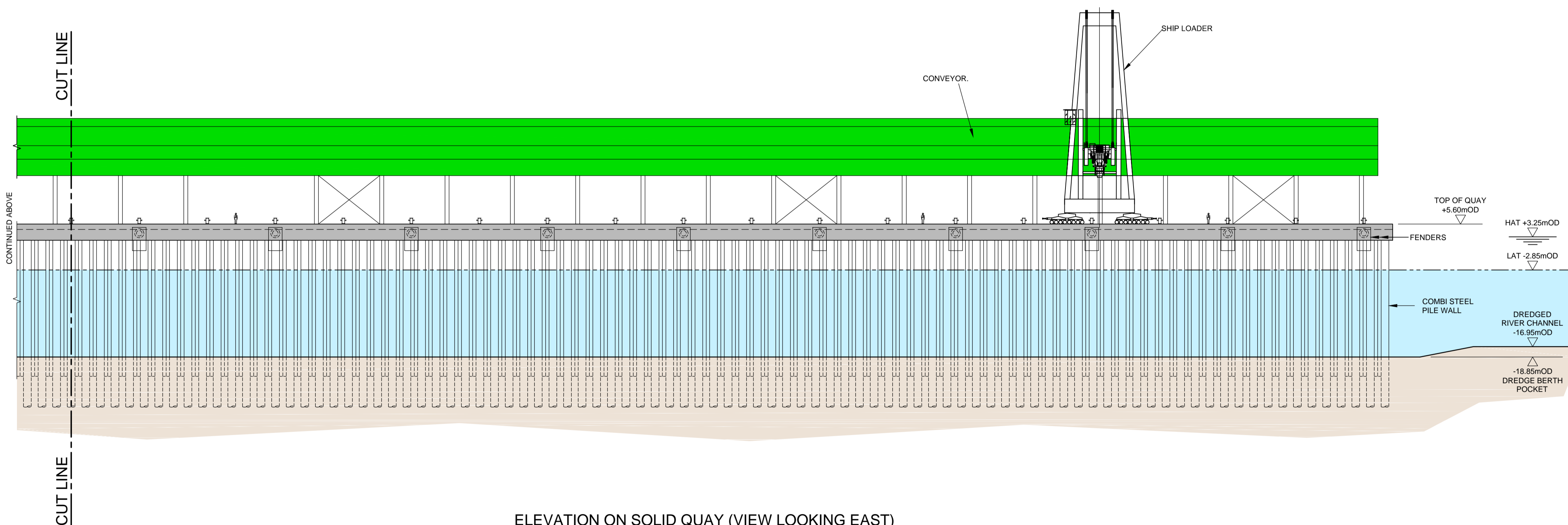
ELEVATION ON SOLID QUAY (VIEW LOOKING EAST)
